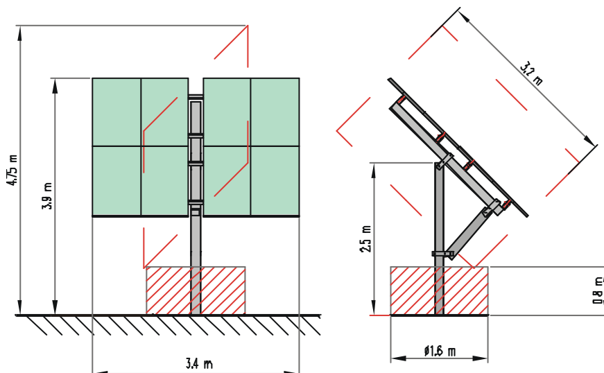
example of system dimensions for 8 x modules BP 3160 (1,280 Wp)
